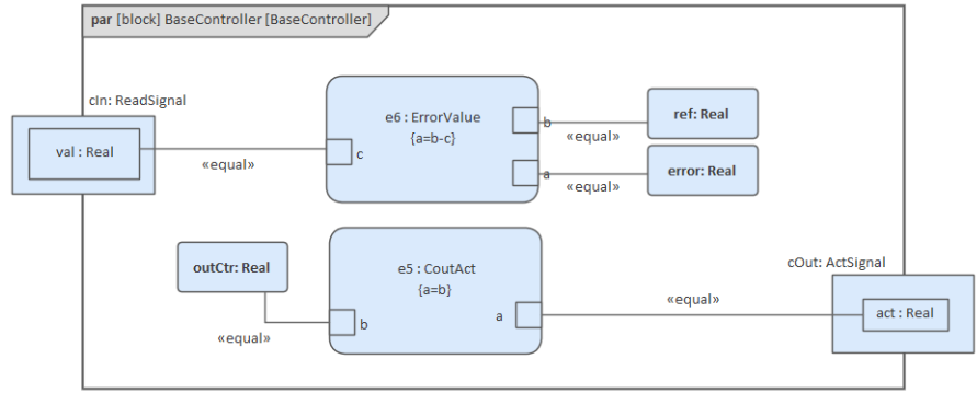
The Constraints defined for 'BaseController' and 'PIcontinuousController' are illustrated in these figures.
